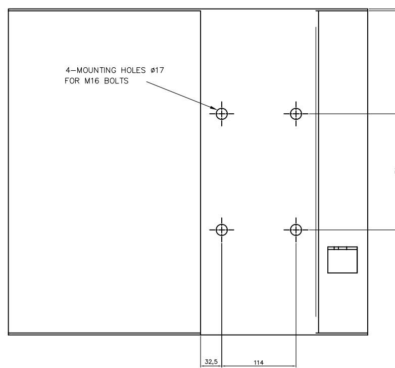
DETAIL OF OUTER COVER ITEM 2 INNER ENCLOSURE NOT SHOWN FOR CLARITY
